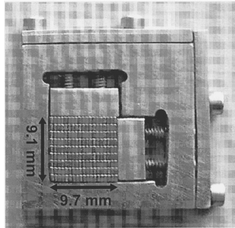
Fig. 1. Photograph of cleaving jig assembly containing 171 copper bars, before nickel and gold metallization, held together in two orthogonal directions with a vise apparatus.
